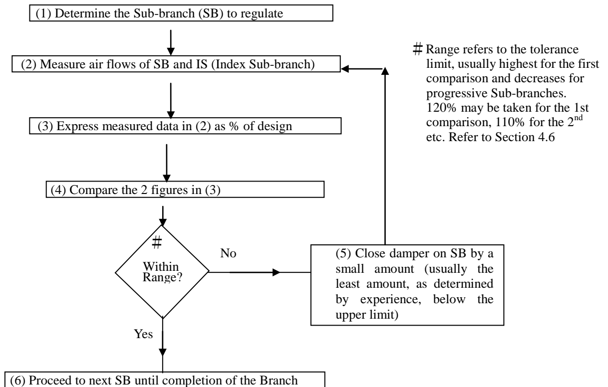
Fig. V3 - Flow chart for Air-balancing of Sub-Branche
